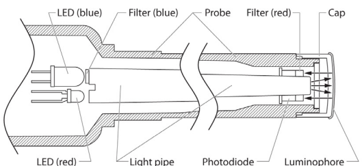
Figure 3 Interior schematic of the Optical DO Probe
