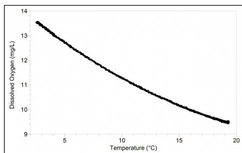
Figure 1 Saturated dissolved oxygen vs. temperature data
