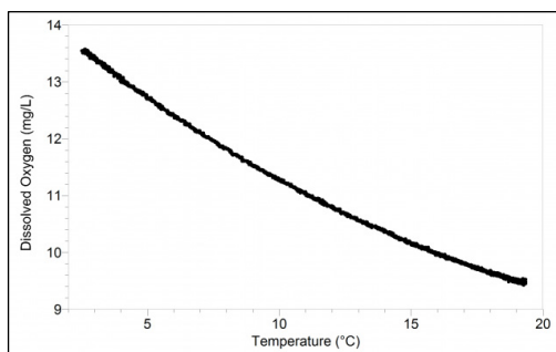
Figure 4 Saturated dissolved oxygen vs. temperature at 760 mmHg
